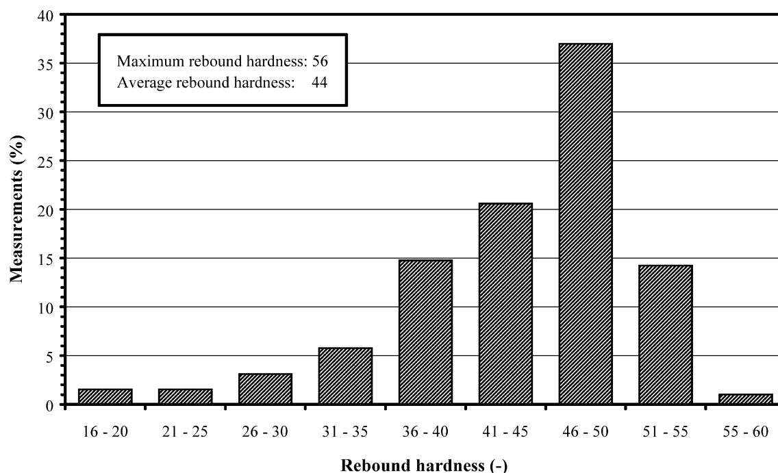
Fig. 20 Classification of the rebound hardnesses
