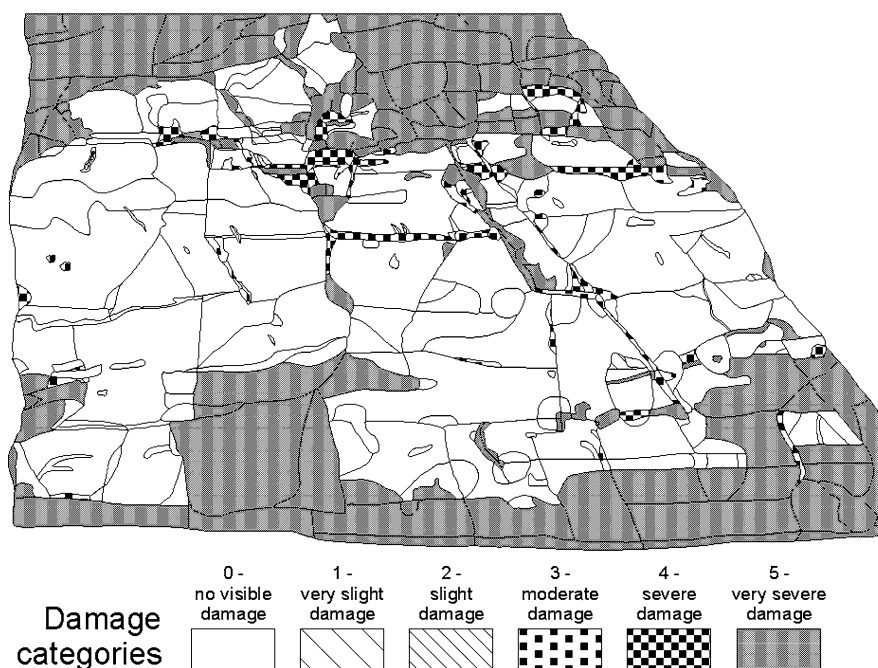
Fig. 13 Damage categories for all weathering forms of group 1 "loss of stone material"
