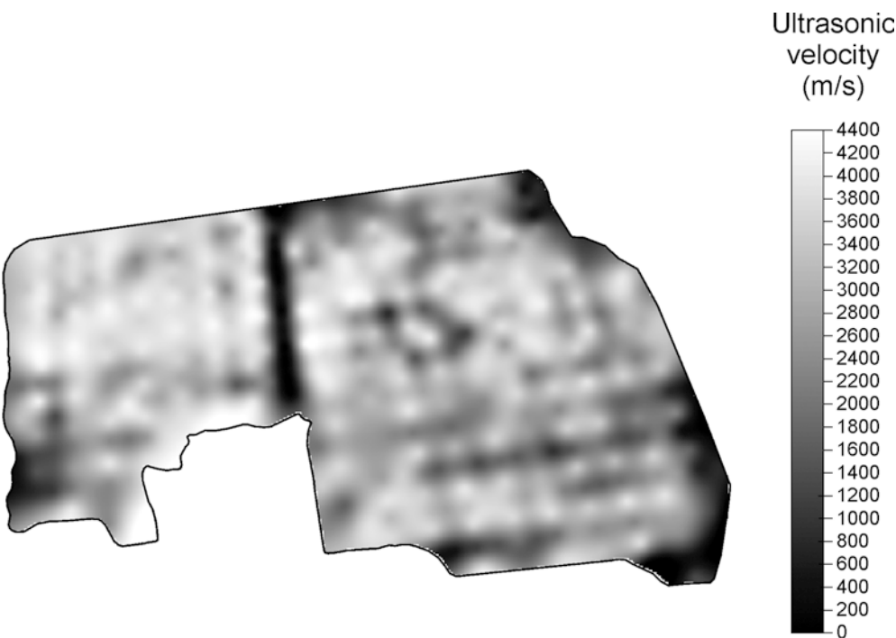
Fig. 17 Ultrasonic measurements. Map of ultrasonic velocities
